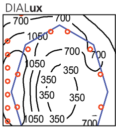
Lighting Diagram Primary Healthcare Trust Reception
