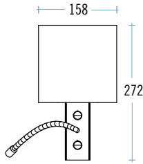
Bedside LED & Shaded Fluorescent
