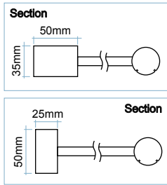
B-line/display/integral35 dimensions B-line/display/integral25 dimensions
