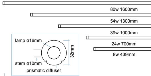
B-line display lengths B-line display shade dimensions
