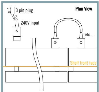
Plug-in system between modules
