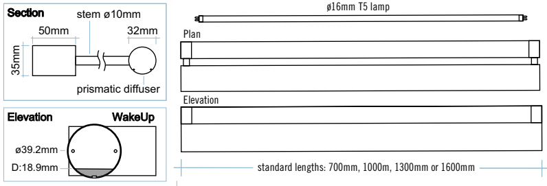
B-line/book/integral35 dimensions WakeUp dimensions
